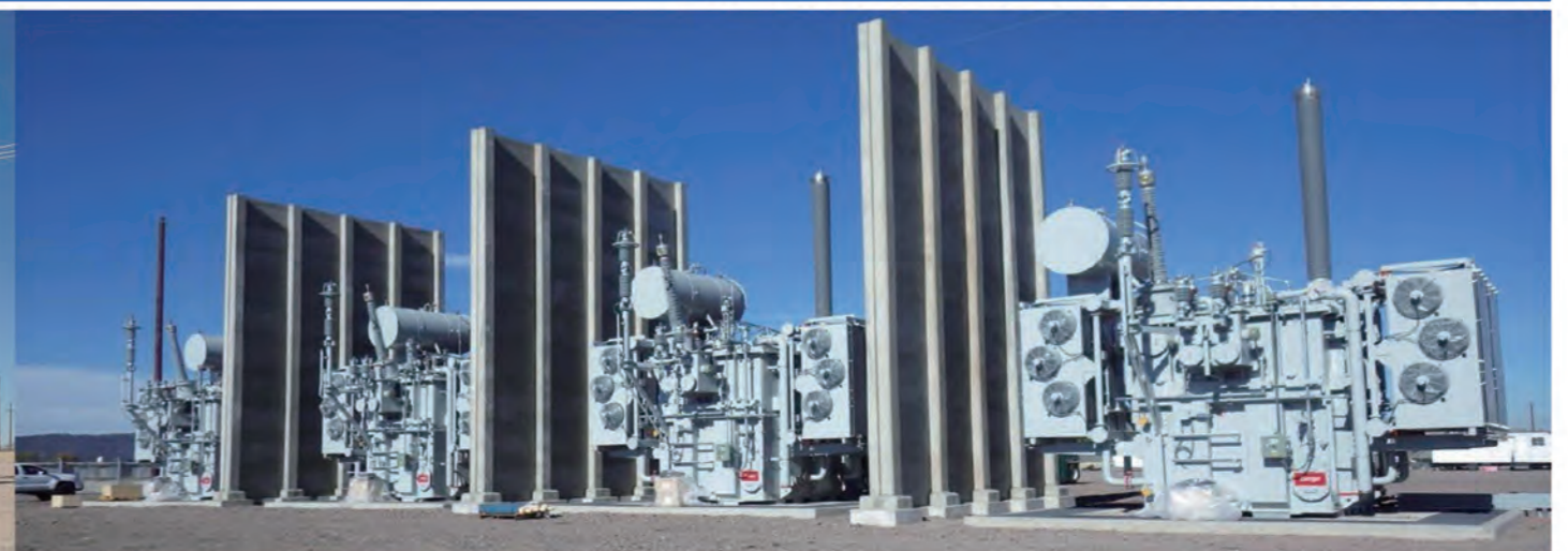
Portland, USA 216.7MVA 525kV Single Phase Power Transformer
